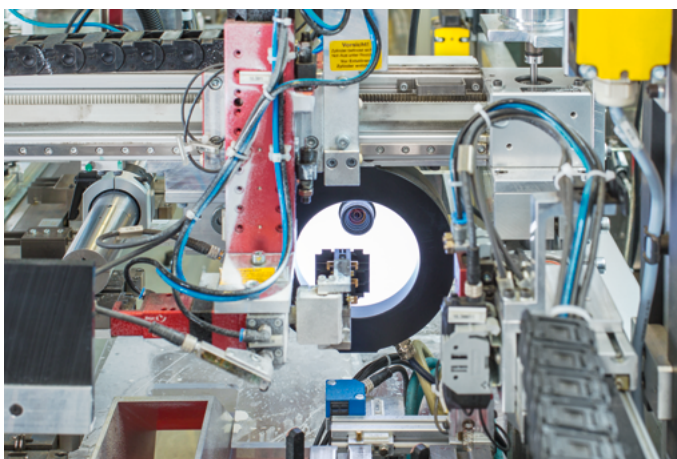
Verification system with LUMIMAX ® Dome Lighting in a production line of Siemens in Amberg
